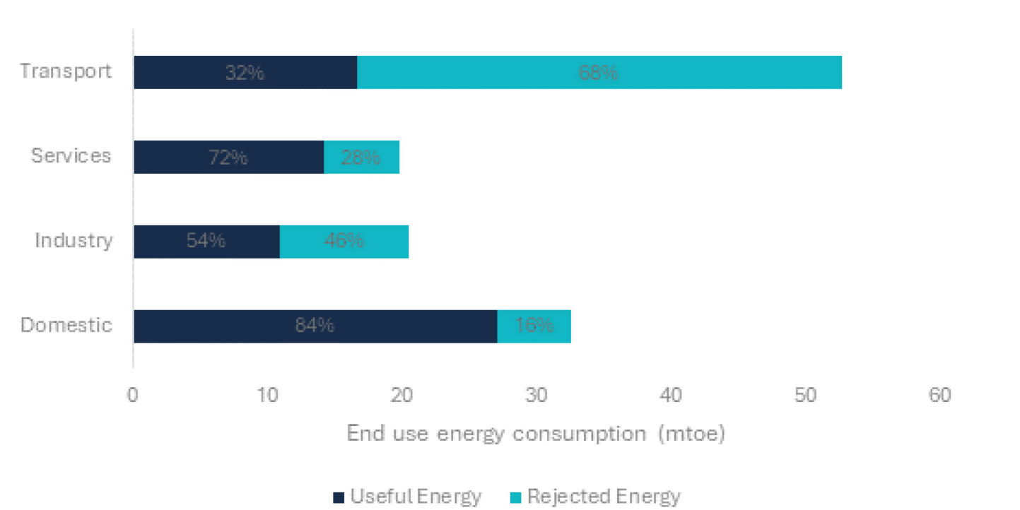
Figure 4: “Useful” and “rejected” energy proportions by sector (mtoe), 2023
