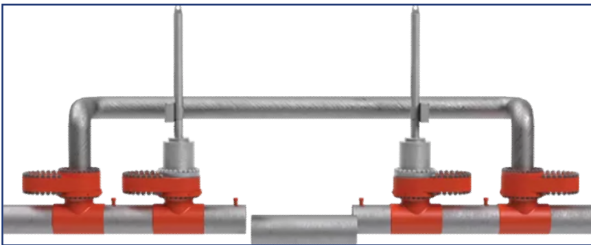
Stopples and bypass arrangement (stopples coloured in red)
