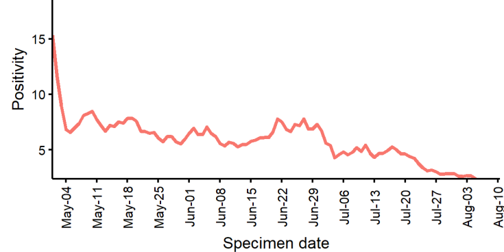
Daily positivity (P1+P2) from May 1 2020
