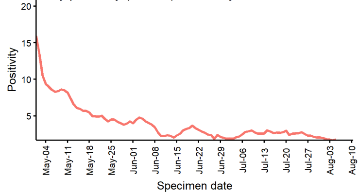
Daily positivity (P1+P2) from May 1 2020
