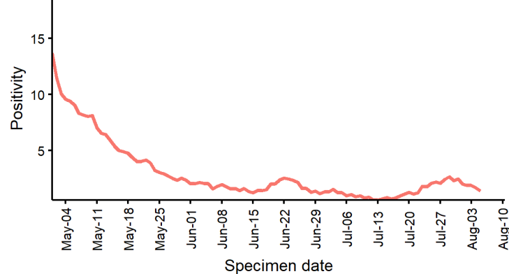
Daily positivity (P1+P2) from May 1 2020
